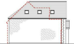
SIDE (NE) ELEVATION
